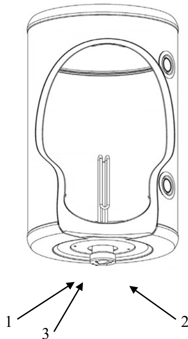
Fig. 2. Installing the electric heater.
