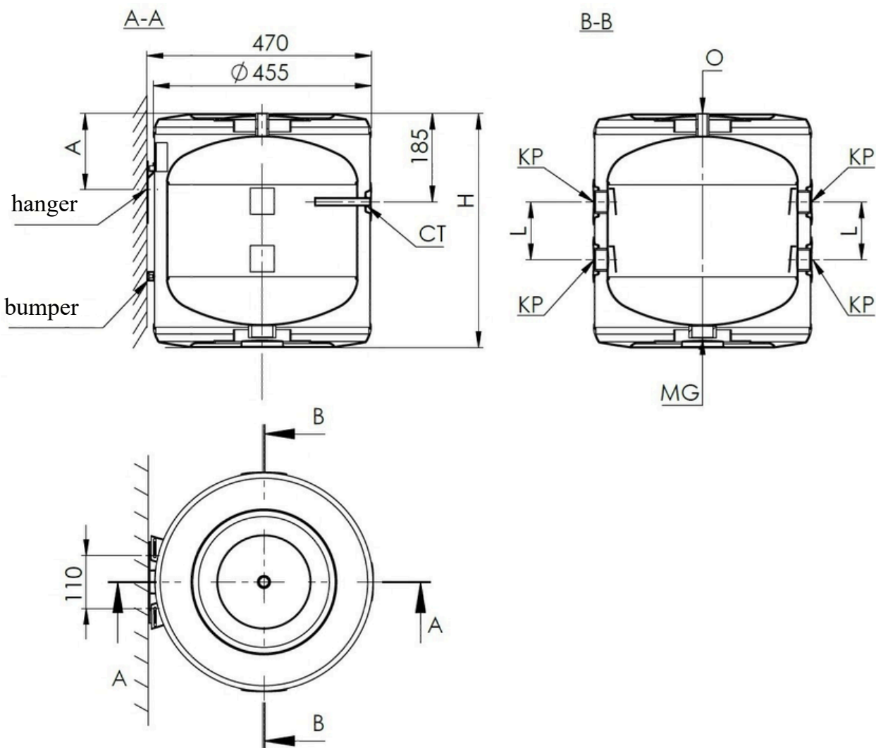
Fig.1 Construction of the NBT-SW buffer tank.
