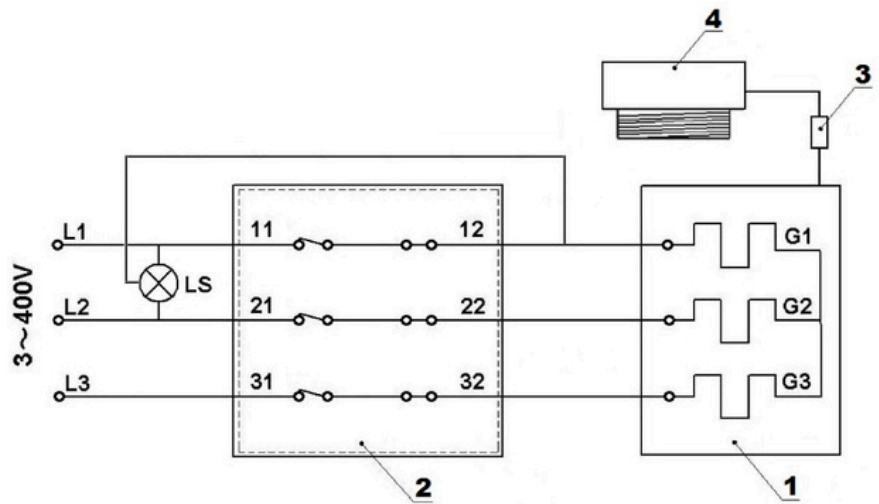
Fig.10 Electrical diagram of a heater with a 3-phase electric heater
