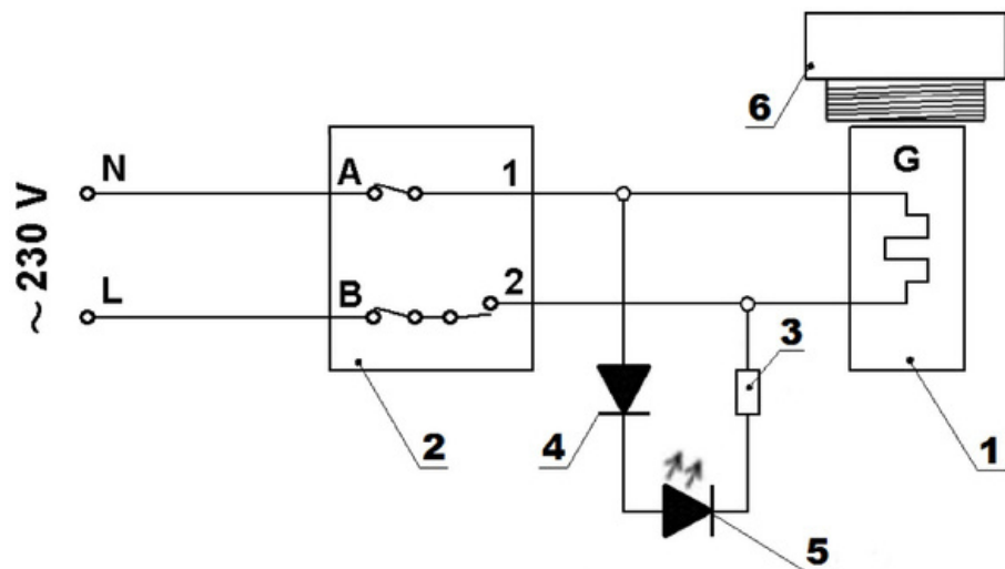
Fig. 9. Electrical diagram of a heater with a 1-phase electric heater.
