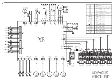
5 Zone System
