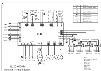
3 Zone System
