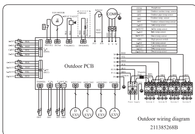
4 Zone System
