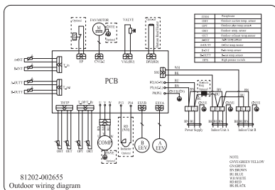
2 Zone System
