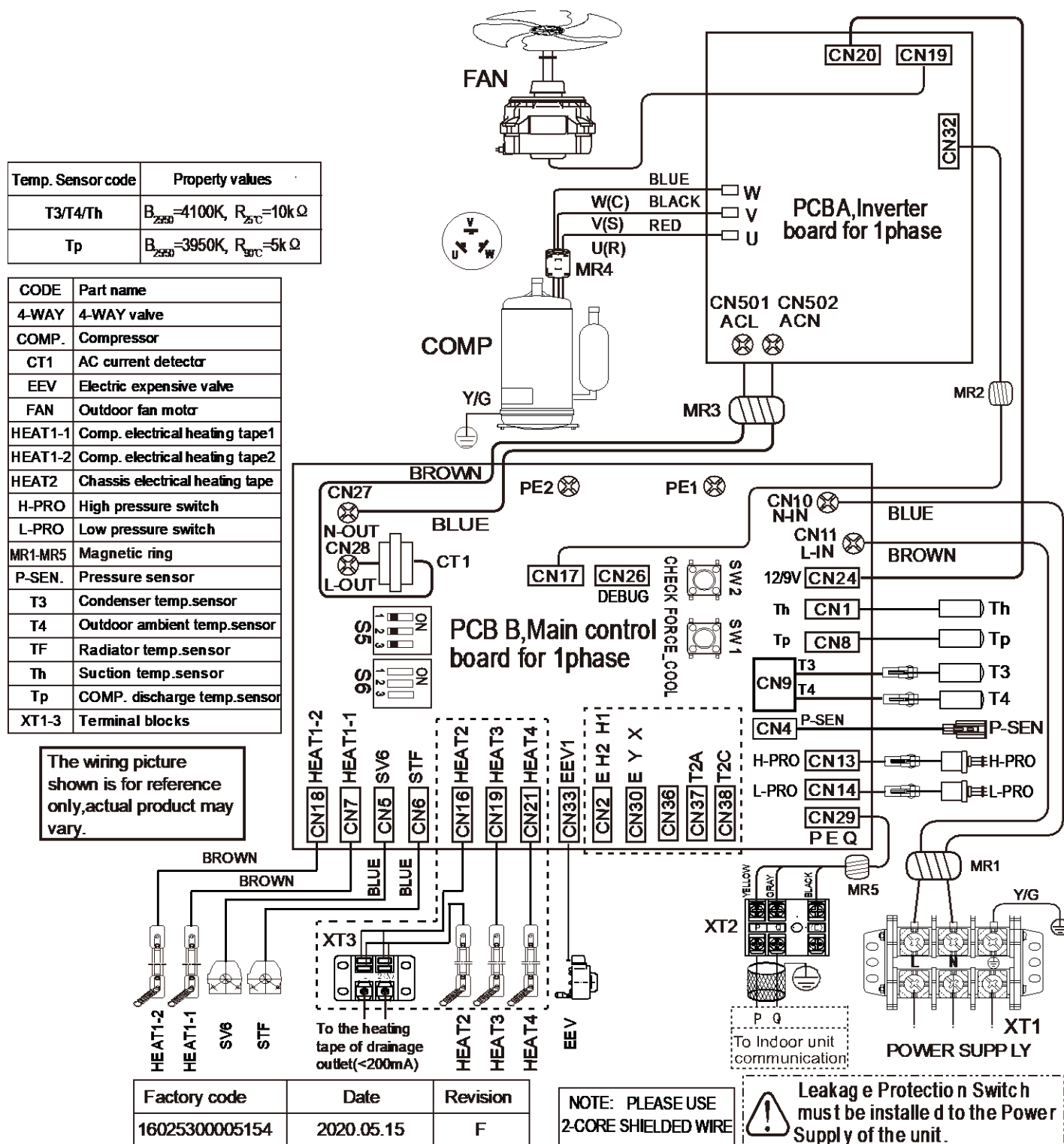
Figure 2-5.1: HOP4(6, 8, 10)WODU wiring diagram
