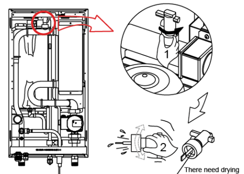
Figure 3-4.2: Water flow switch
