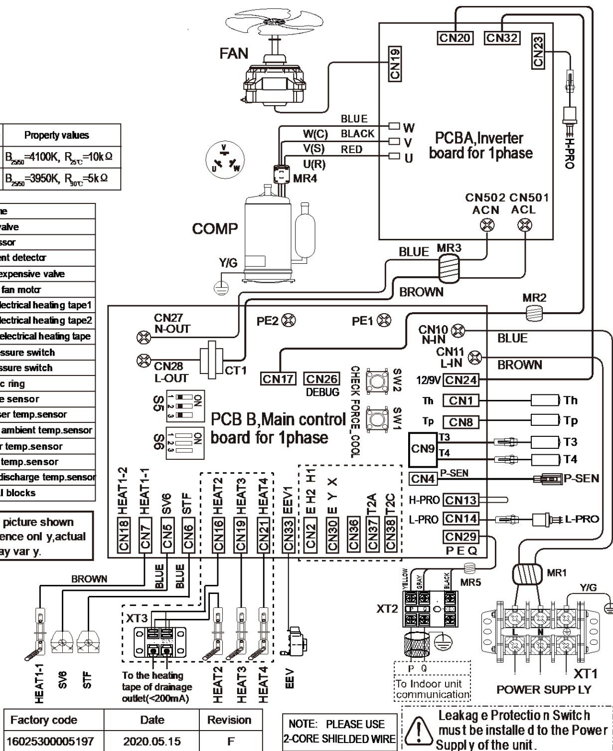
Figure 2-5.1: HOP12(14,16)WODU wiring diagram
