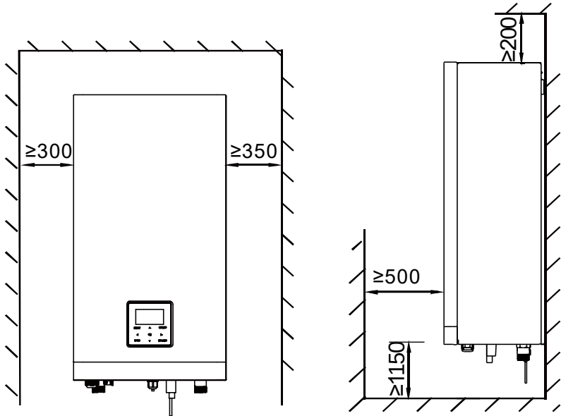
Figure 3-2.15: Service space requirement (unit:mm)
