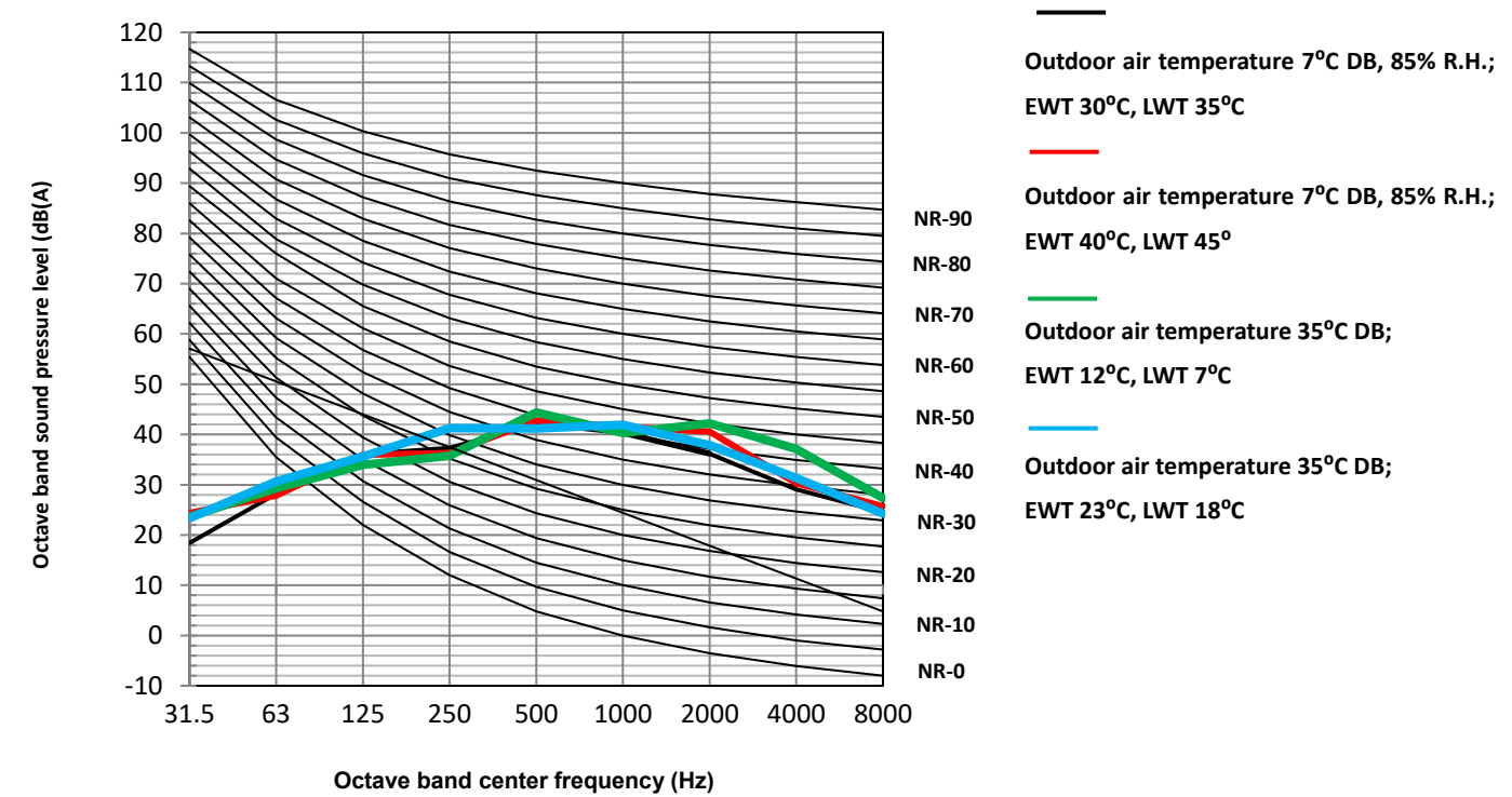
Figure 2-9.3: HOP6WODU octave band levels
