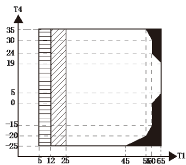
Figure 2-7.1: Heating operating limits 1
