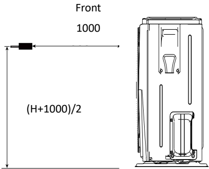
Figure 2-8.1: Sound pressure level measurement (unit: mm)
