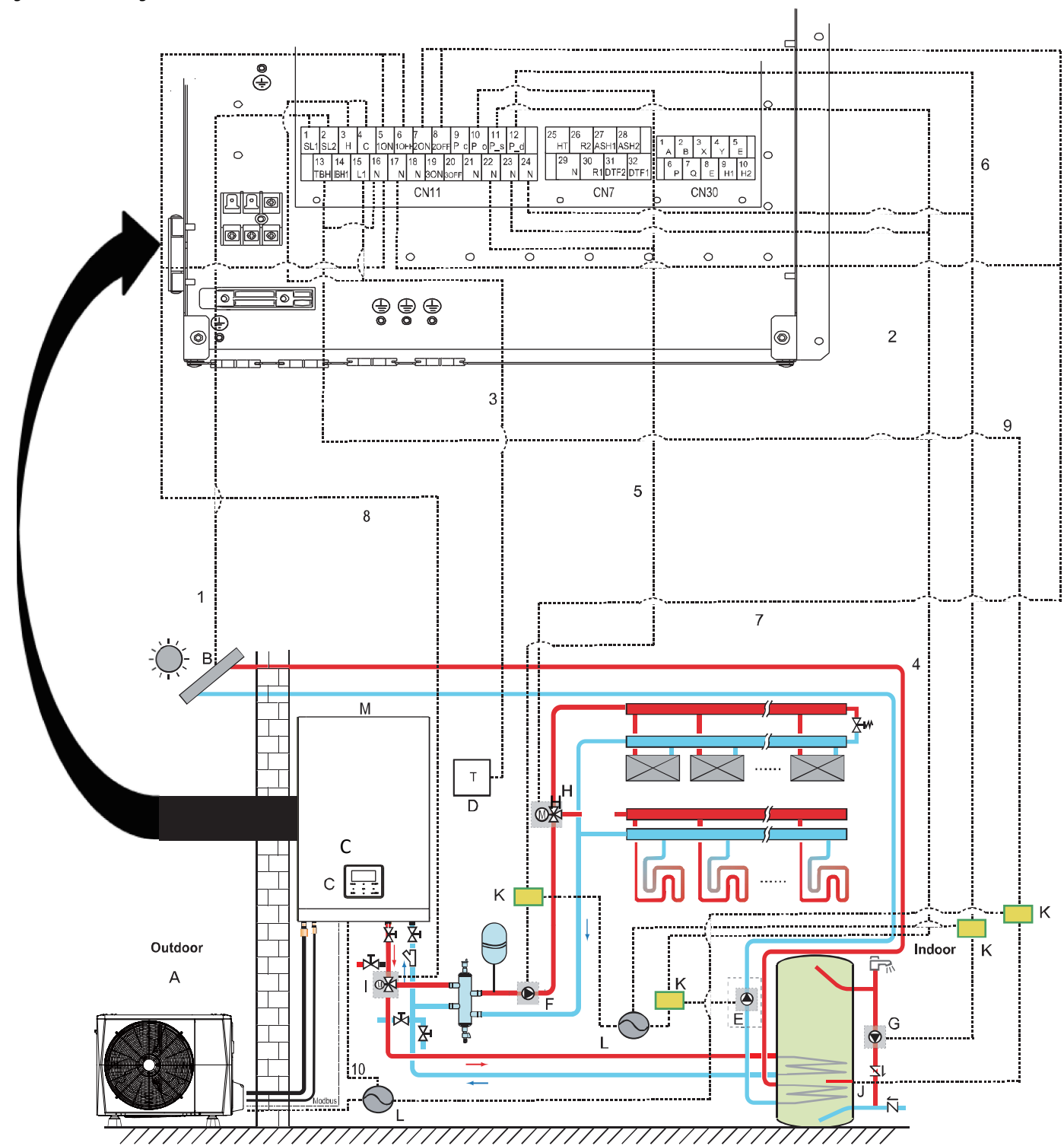
Figure 3-5.1: Wiring overview
