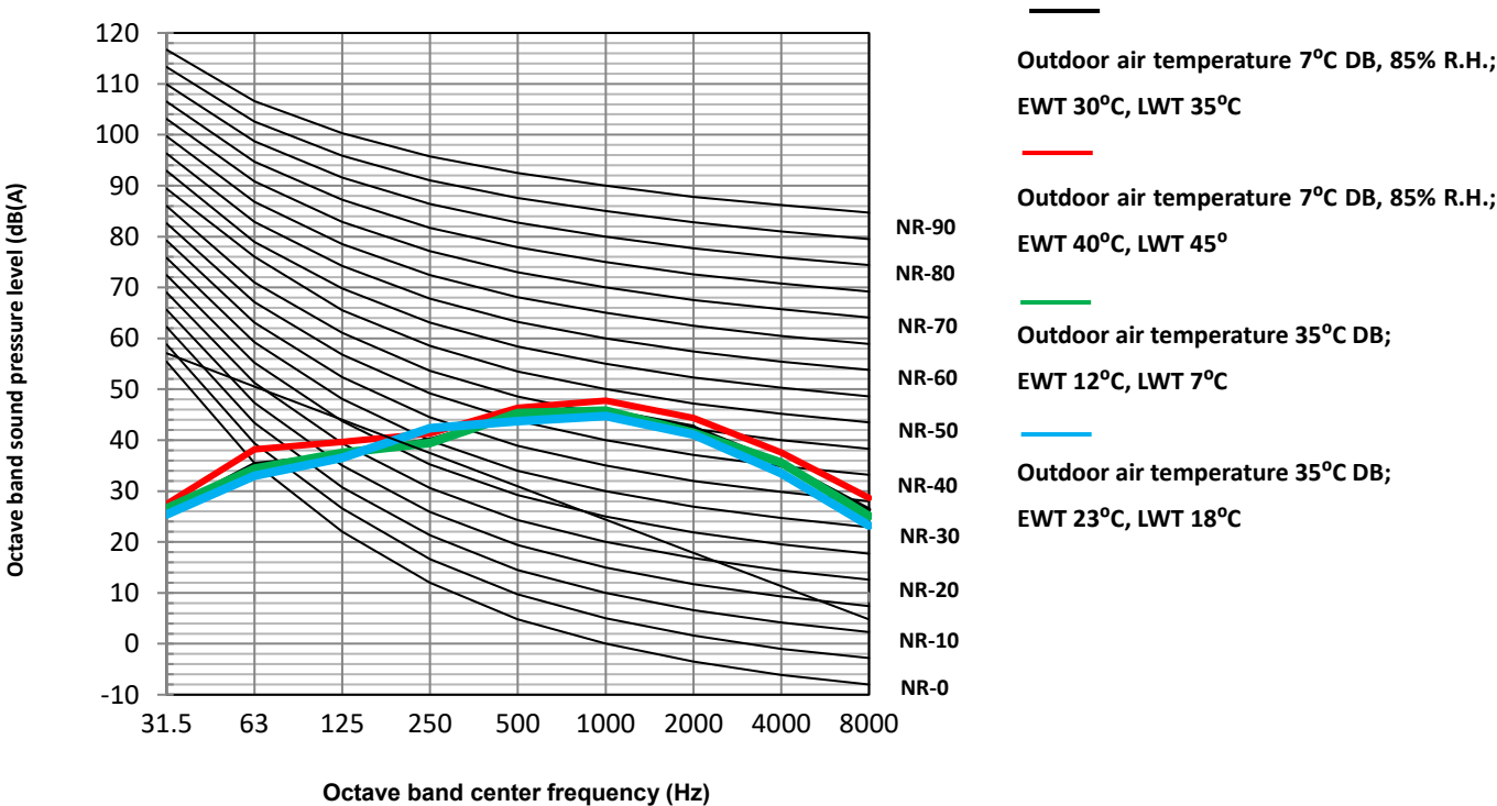
Figure 2-9.5: HOP10WODU octave band levels
