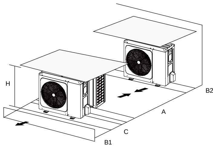
Figure 3-2.10: Single row installation
