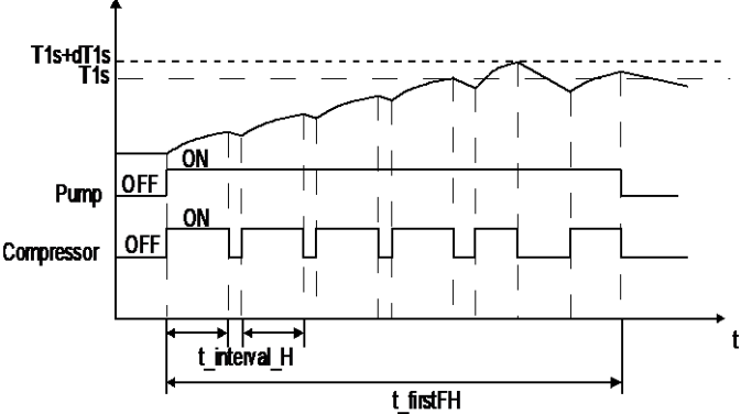
Figure 3-8.42: Preheating for floor
