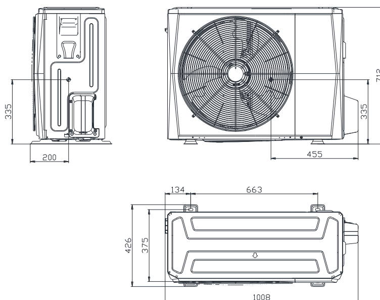
Figure 2-3.1: Dimensions and center of gravity (unit: mm)
