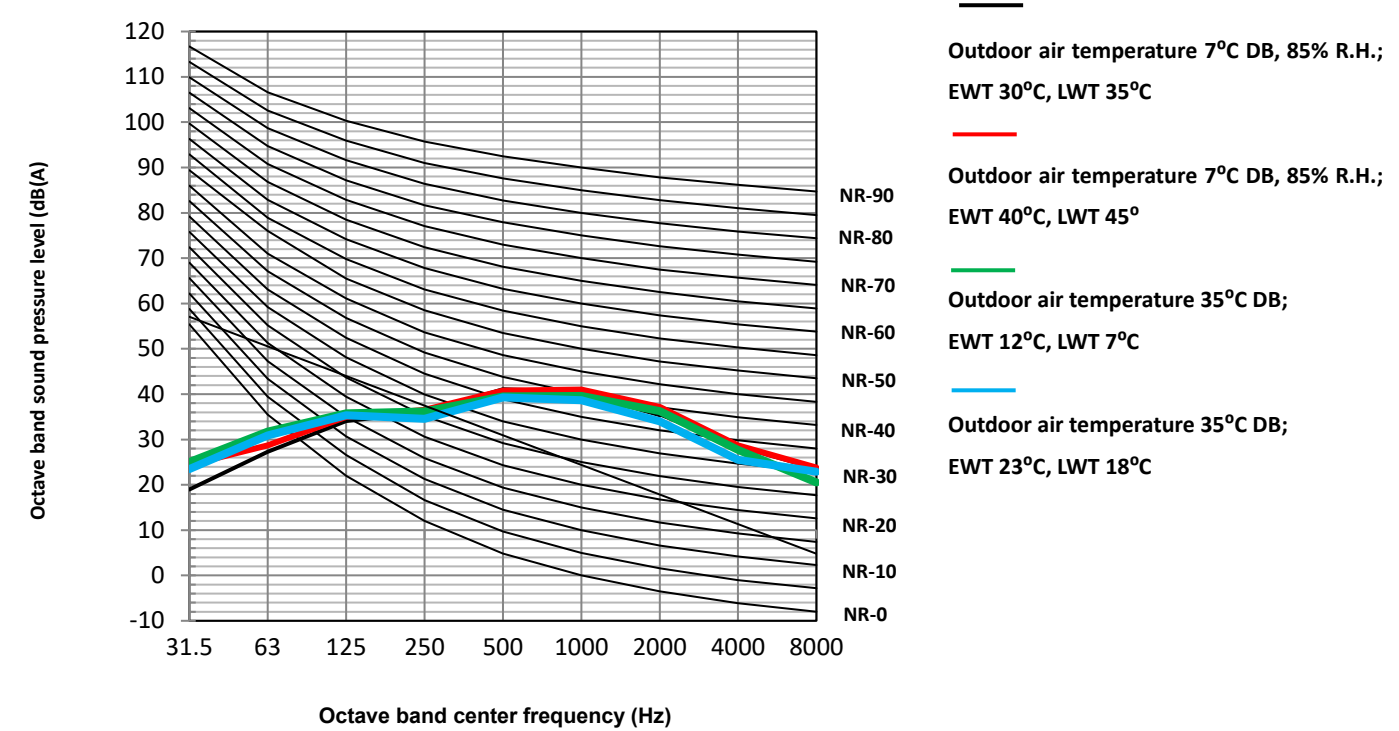
Figure 2-9.2: HOP4WODU octave band levels
