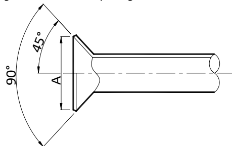
Figure 3-3.3: Flared opening
