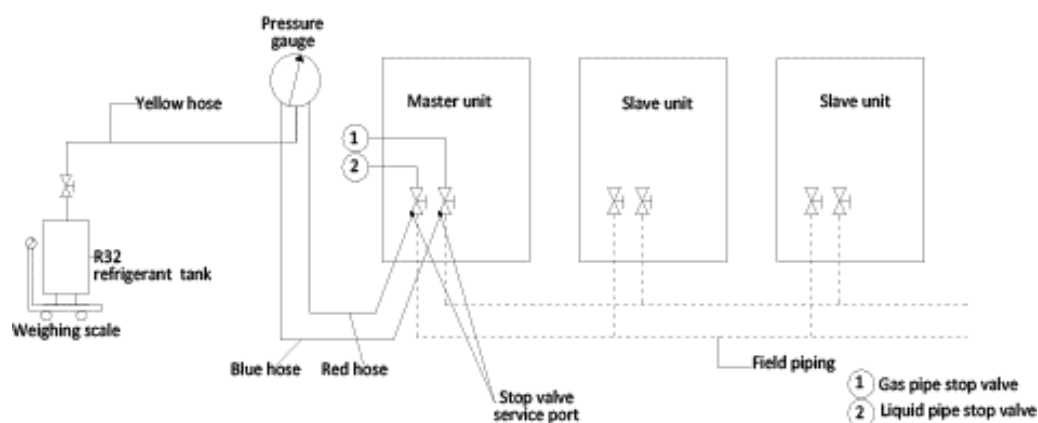
Figure 3-3.13: Charging refrigerant
