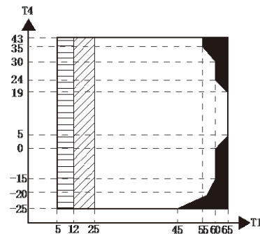
Figure 2-7.3: Domestic hot water operating limits 1
