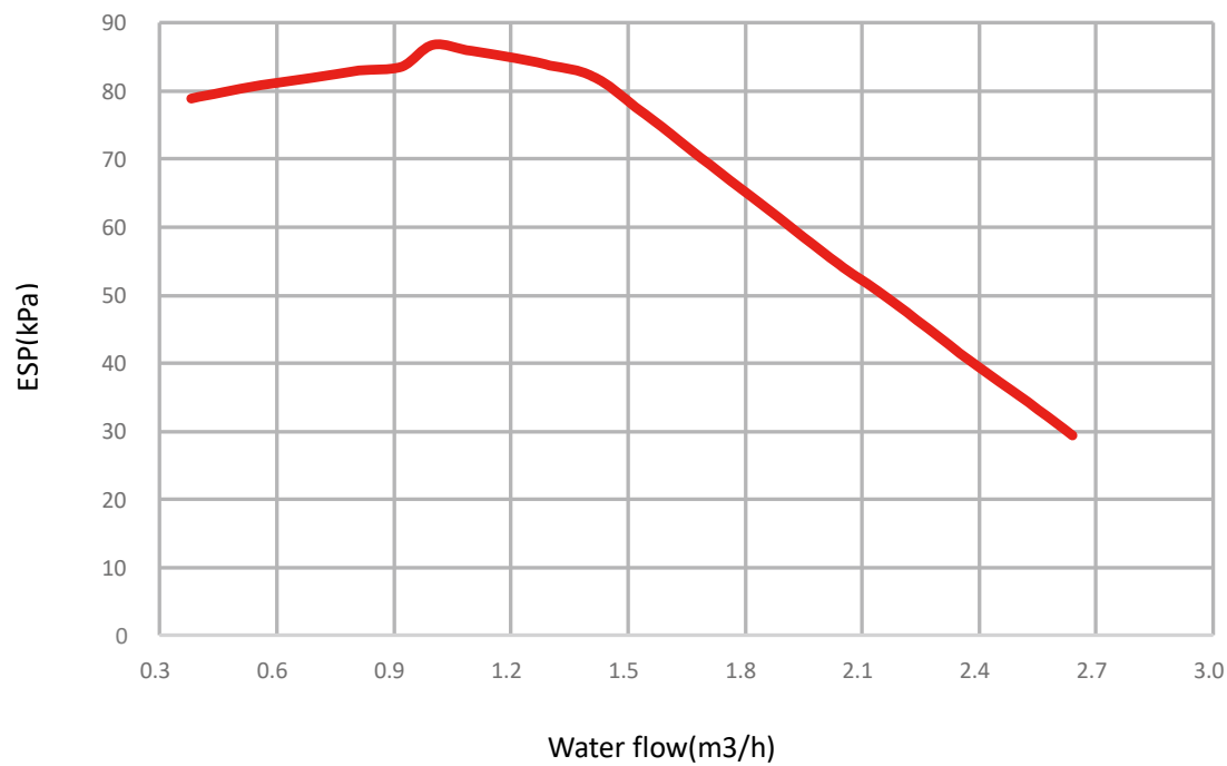
Figure 2-8.2: HOP160WIDU3 hydronic performance
