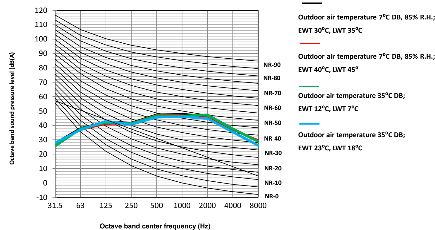
Figure 2-9.5: HOP14WODU octave band levels
