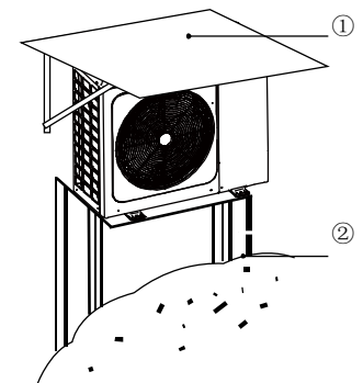
Figure 3-2.2: Snow shielding
