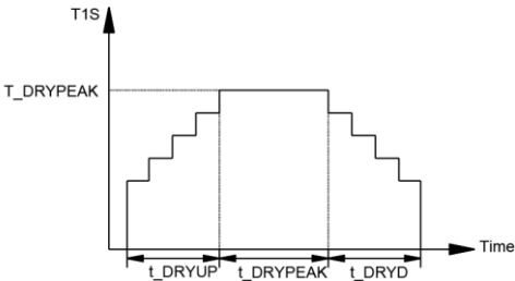
Figure 3-8.45: FLOOR DRYING UP settings
