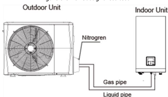
Figure 3-3.10: Gastightness test
