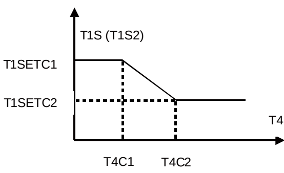
Figure 3-12.7: Automatic setting curve for cooling mode
