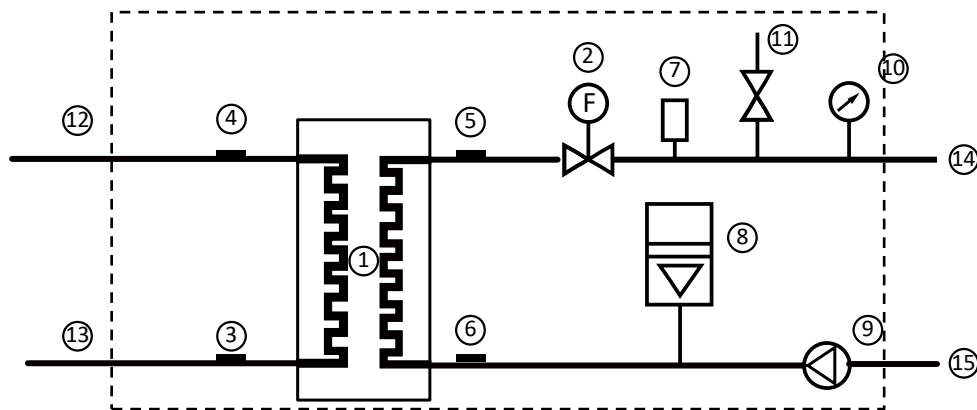
Figure 2-4.2:Hydronic box piping diagram
