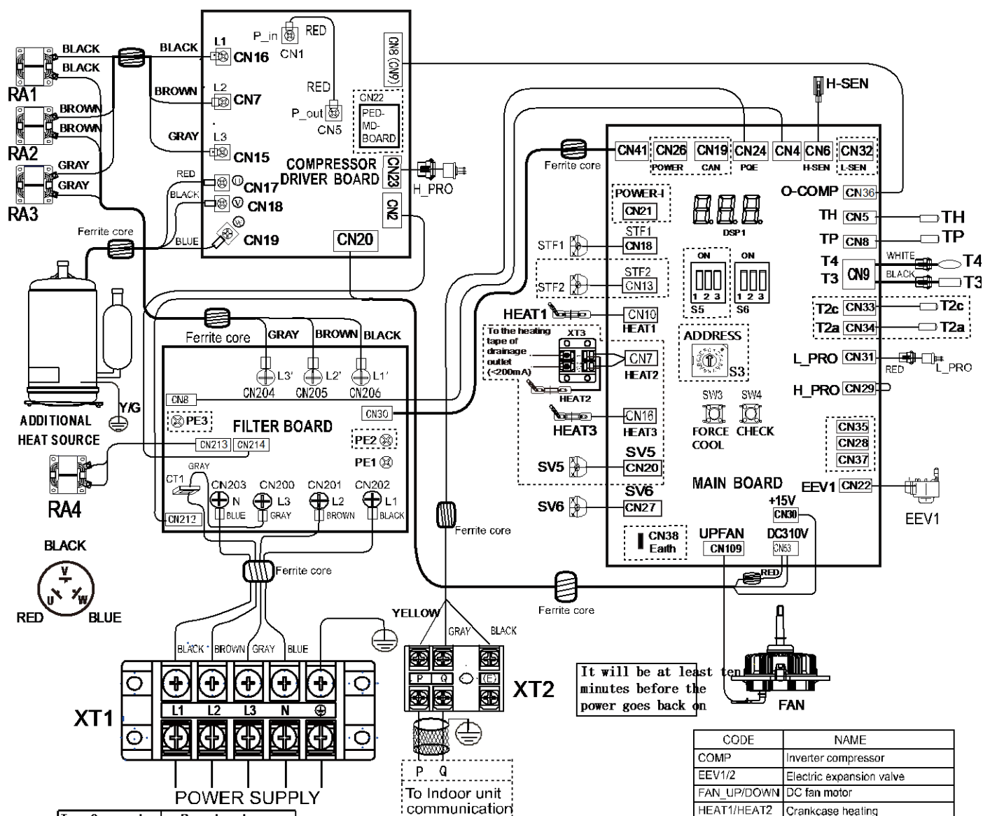
Figure 2-5.1: HOP12(14,16)WODU3 wiring diagram
