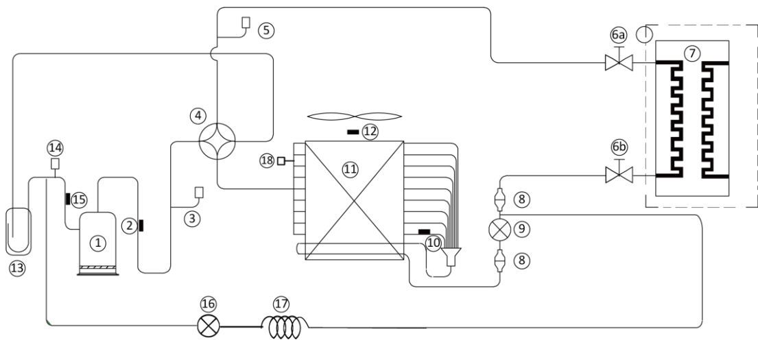
Figure 2-4.1: Outdoor unit piping diagram
