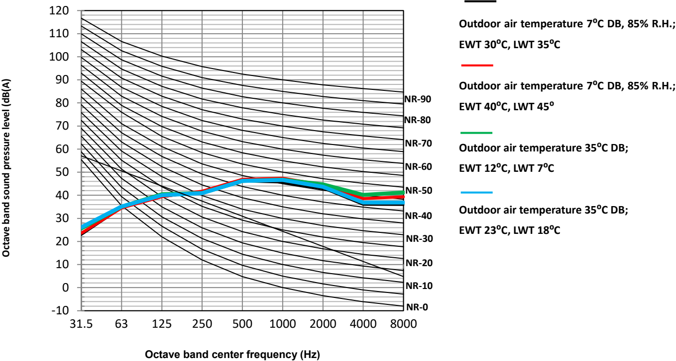
Figure 2-9.5: HOP12WODU3 octave band levels
