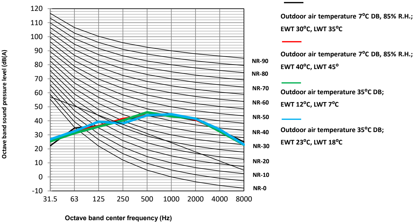
Figure 2-9.4: HOP8WODU octave band levels
