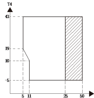
Figure 2-6.2: Cooling operating limits
