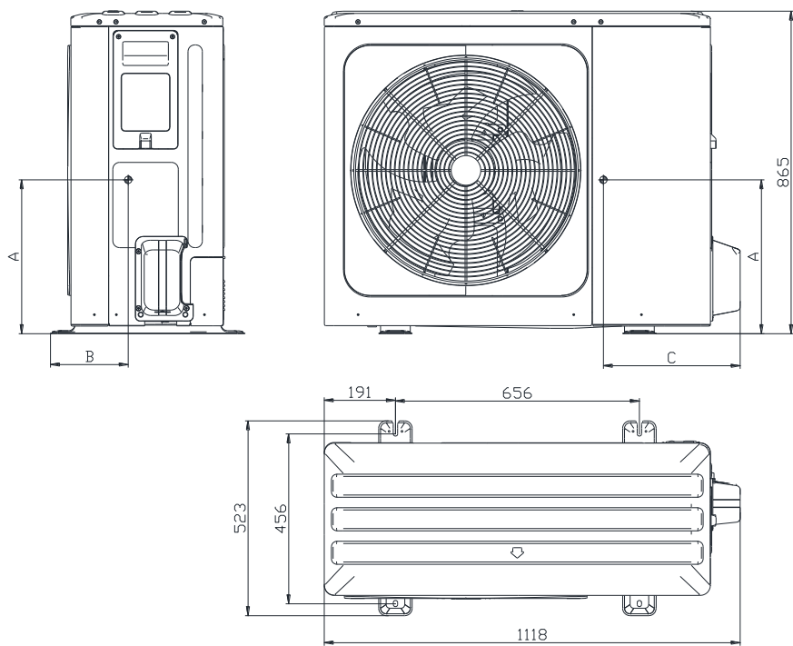
Figure 2-3.2: Dimensions and center of gravity (unit: mm)
