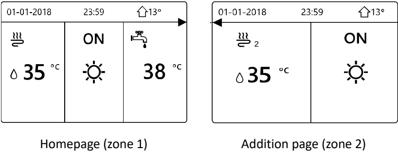
Figure 3-8.23: Set DOUBLE ZONE to YES and set ROOM TEMP. to NON; Set WATER FLOW TEMP. to YES or NON
