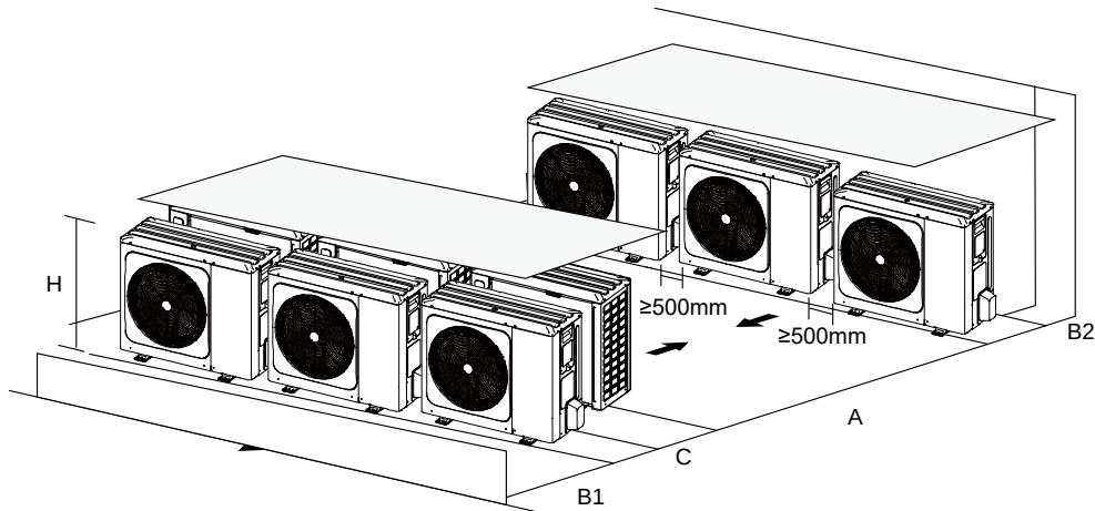
Figure 3-2.11: Multi-row installation
