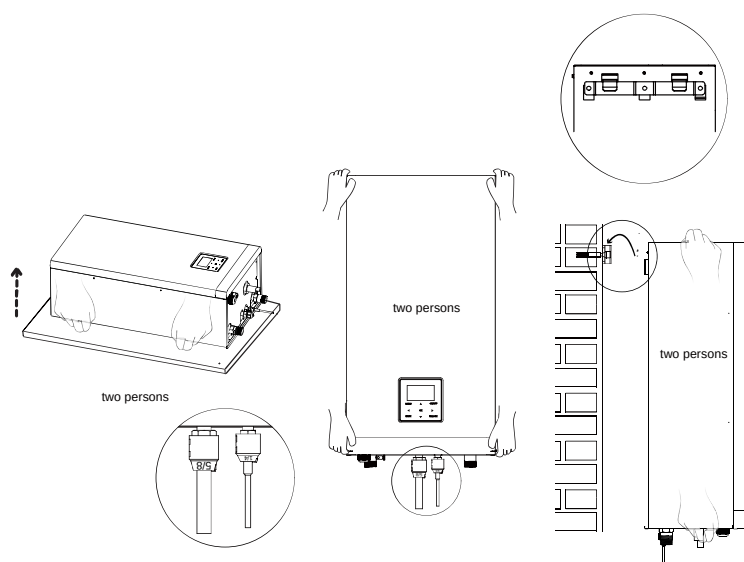
Figure 3-2.14: Fix hydronic box
