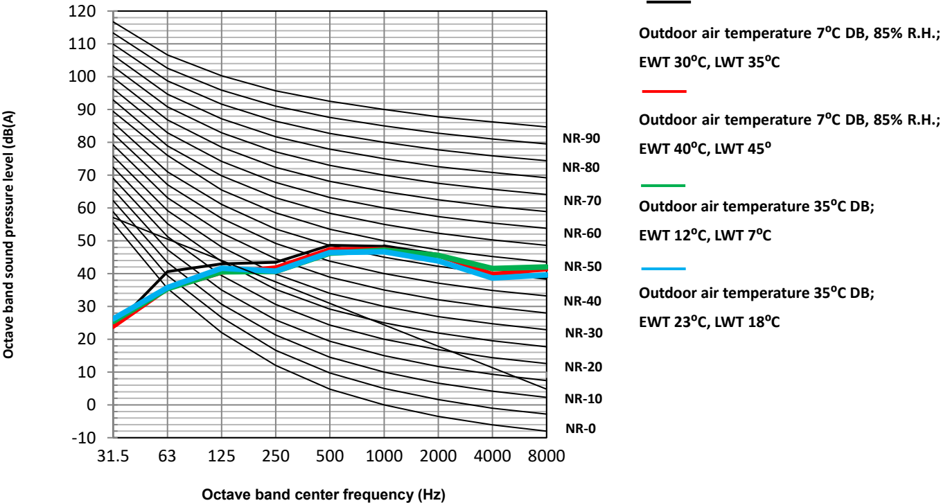
Figure 2-9.5: HOP14WODU3 octave band levels
