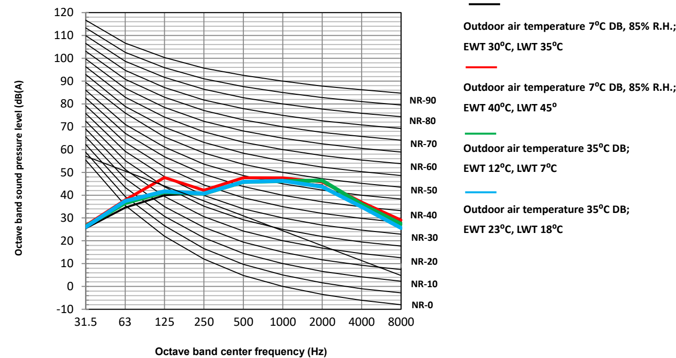
Figure 2-9.5: HOP12WODU octave band levels
