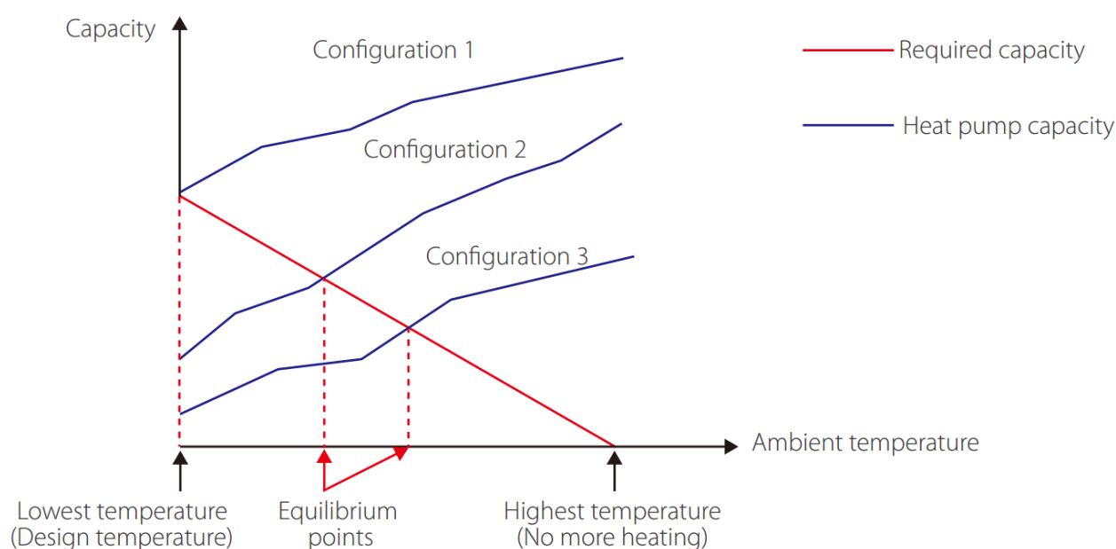
Figure 1-1.2: System configurations
