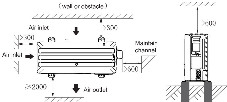
Figure 3-2.7: Single unit installation requirement (Unit: mm)
