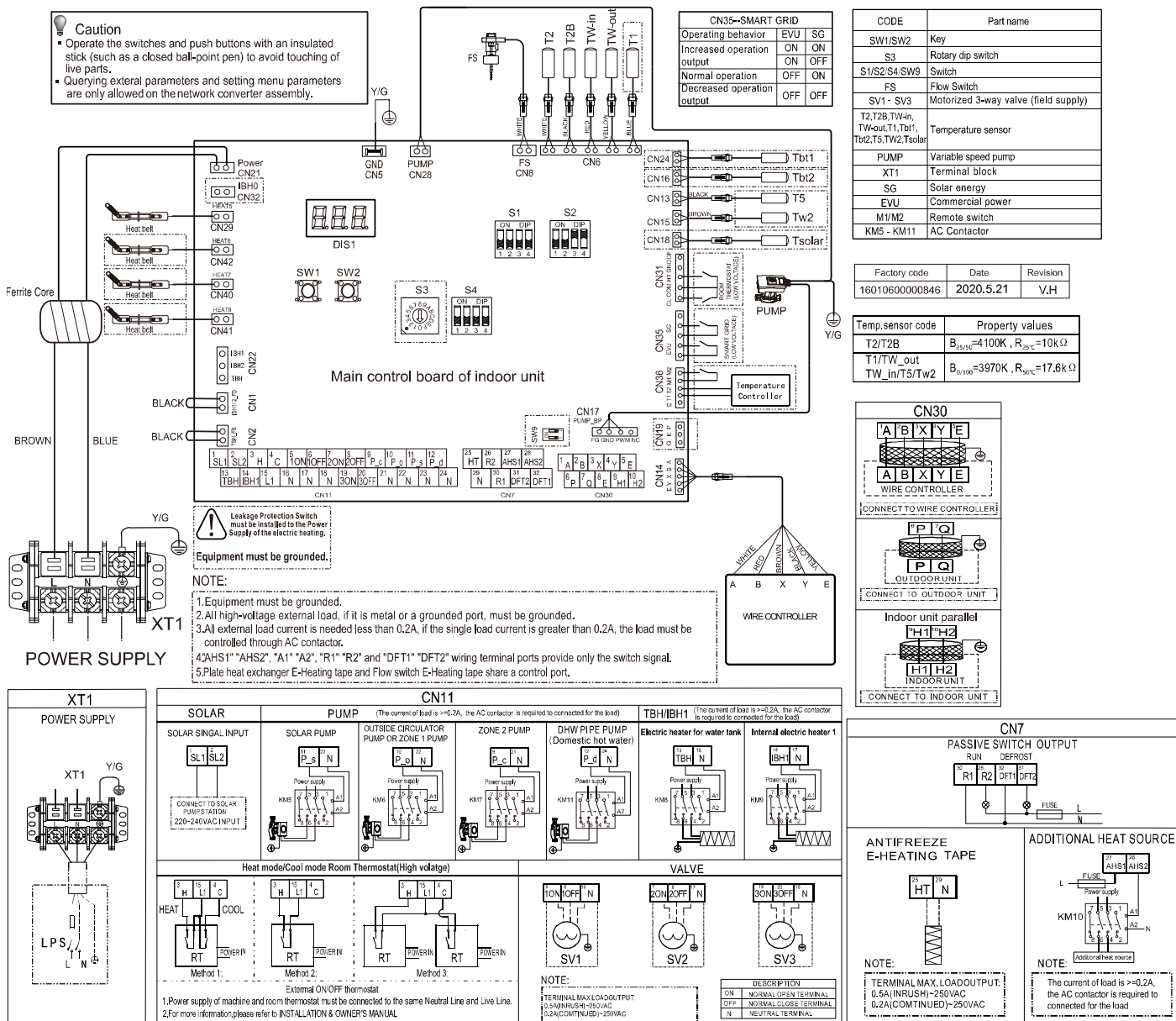
Figure 2-5.2 HOP60(100,160)WIDU(3) wiring diagram
