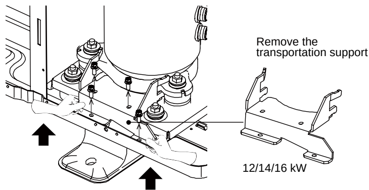
Figure 3-2.6: 12-16kW models 2.3.7 transportation support
