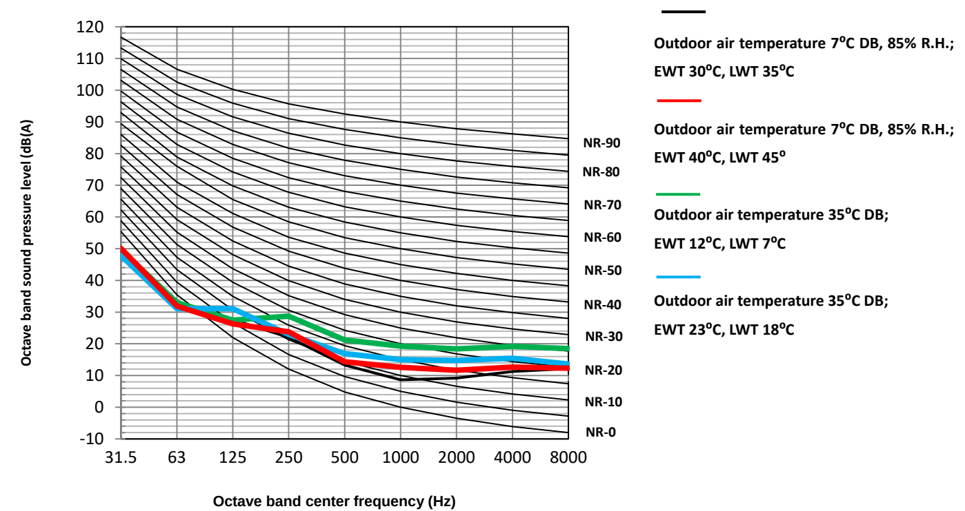
HOP6WODU + HOP100/190IDU(3) (3/9kW) octave band levels
