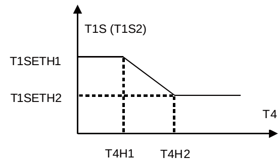
Automatic setting curve for heating mode
