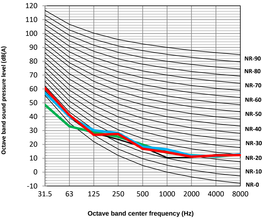
HOP12WODU(3) + HOP160/240IDU (9kW) octave band levels
