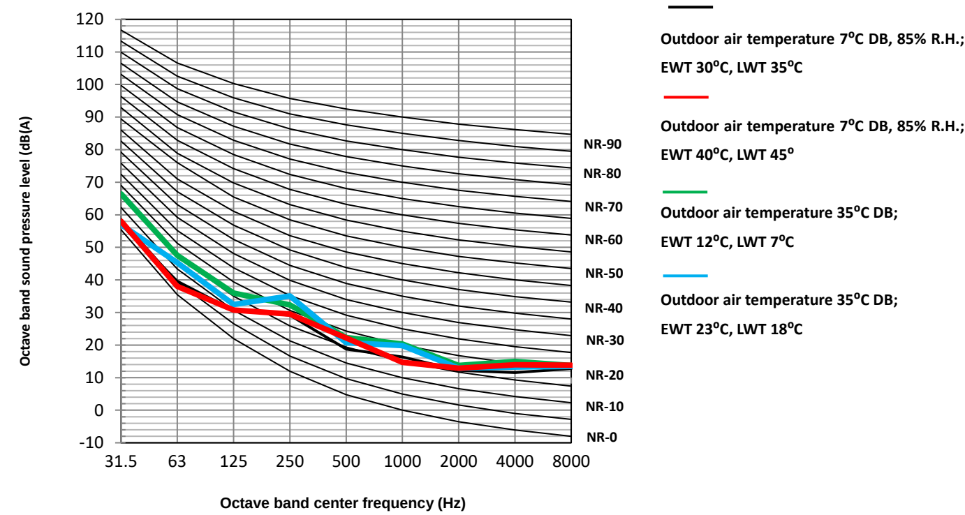
HOP14WODU(3) + HOP160/240IDU (9kW) octave band levels
