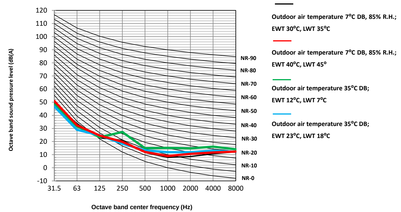
HOP4WODU + HOP100/190IDU(3) (3/9kW) octave band levels
