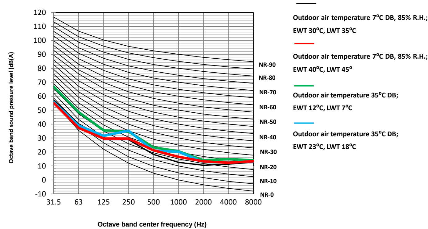
HOP16WODU(3) + HOP160/240IDU (9kW) octave band levels
