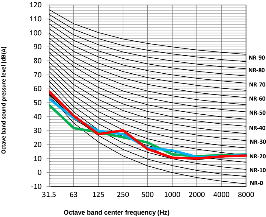
HOP8(10)WODU + HOP100/190IDU(3) (3/9kW) octave band levels
