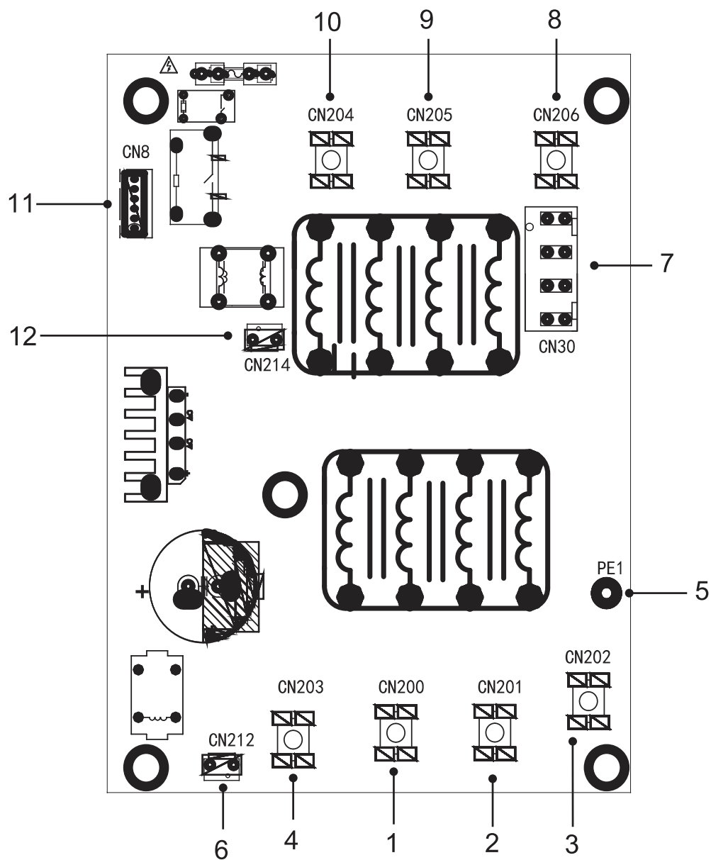
PCB C
